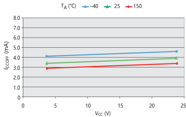
Supply Current (Off) versus Supply Voltage
